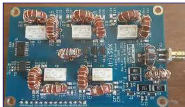
Figure 4 : RF board component side
